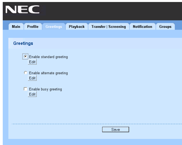
Figure 32. Greetings Screen
