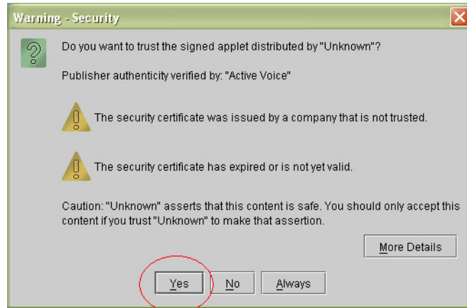
Figure 15. Security Screen
