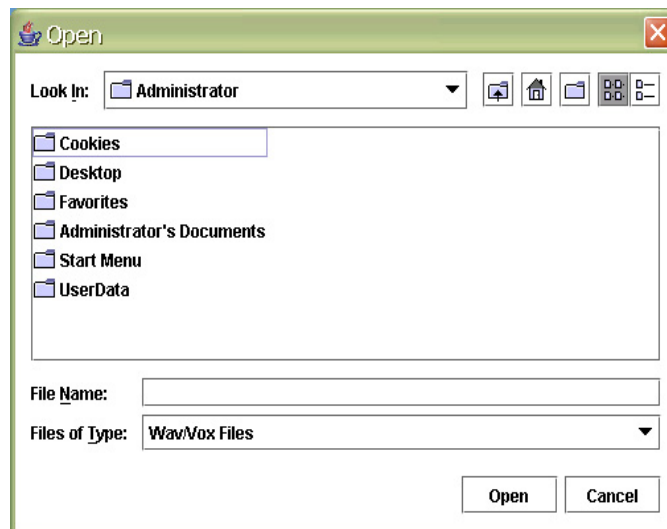
Figure 30. Browse Window
